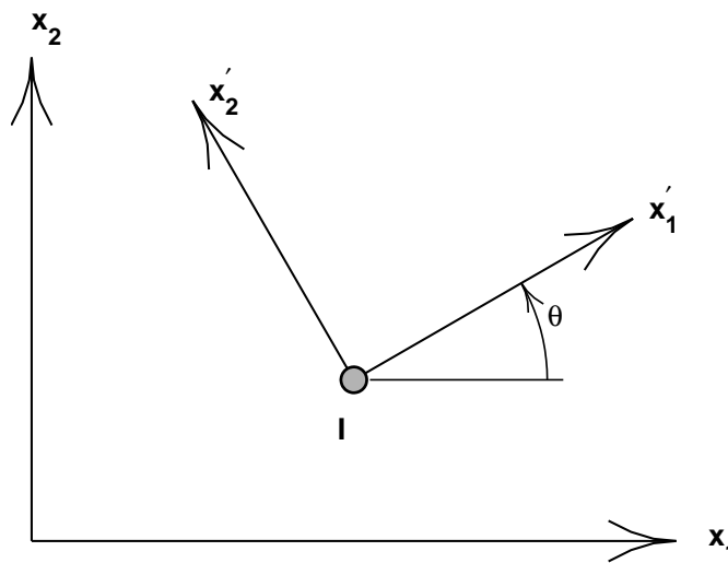
Figure A.6: Coordinate rotation for node I.
